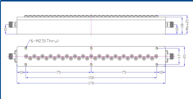
Outline Tolerances ±0.5mm (0.02inch)
