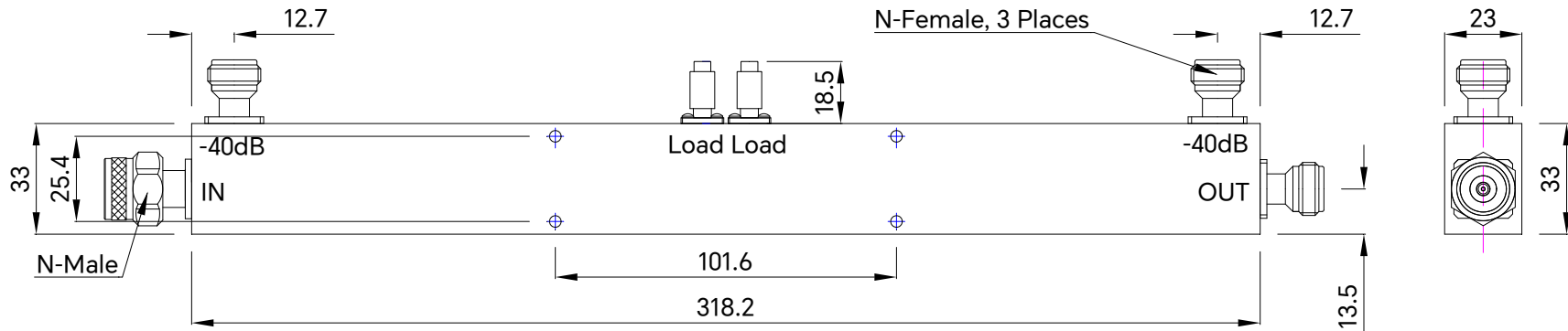
Drawing not to scale, units:mm
