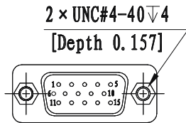
DB15 male
