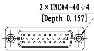
DB26 male
