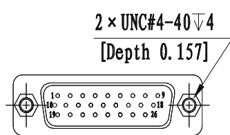
DB26 male
