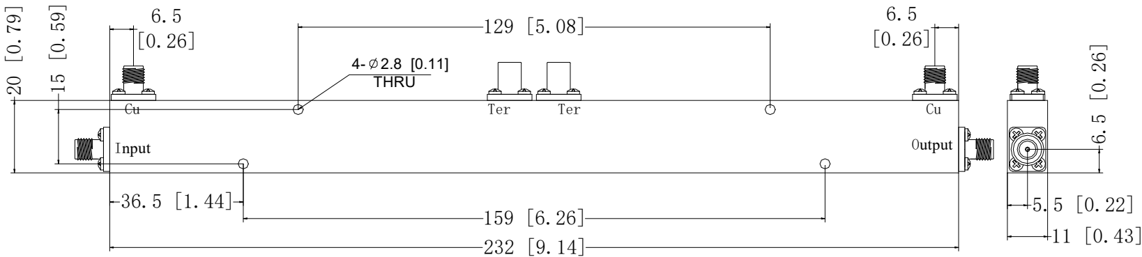
Drawing not to scale, units:mm
