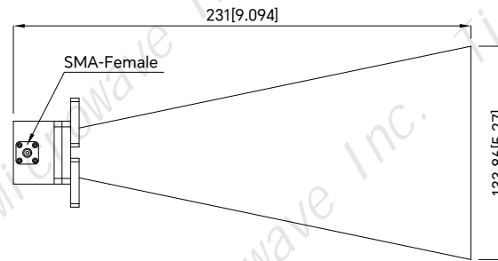
Outline Drawing With Mounting Bracket
